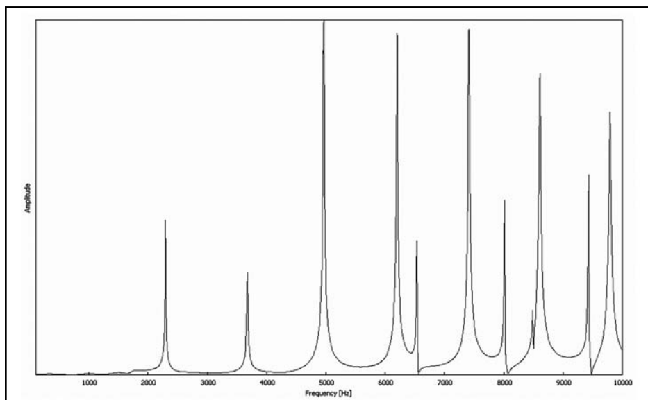
Fig 6: Spectrum at \alpha = 180^\circ , giving \theta = 90^\circ between speaker and microphone
