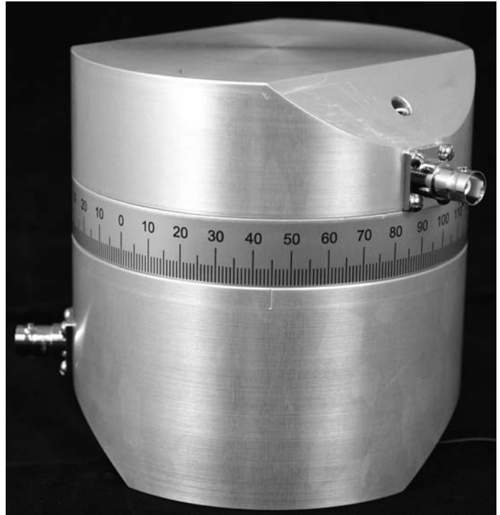
Fig 1: The "Hydrogen Atom"
