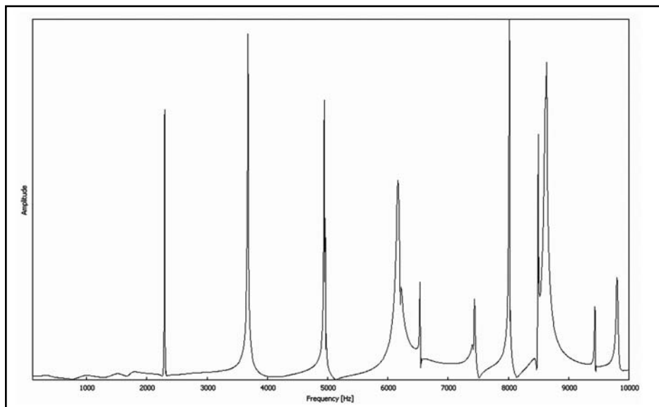
Fig 5: Spectrum \alpha = 0^\circ , giving \theta = 90^\circ between speaker and microphone
