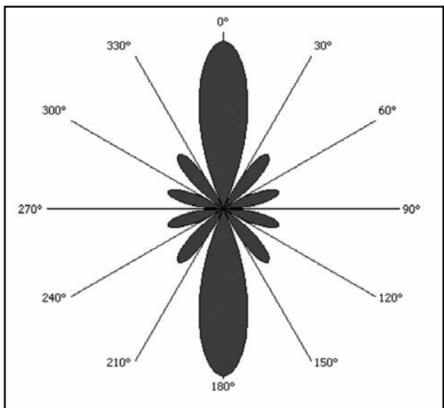
Fig 4: Wavefunction of the peak at about 7460Hz (left) and calculated spherical harmonics for l = 5, m = 0 (right).
