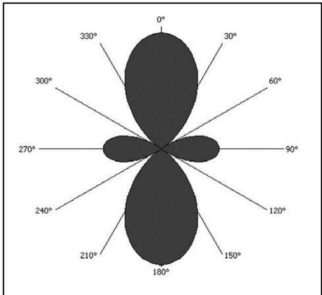
Fig 3: Wavefunction of the peak at about 8040Hz that belongs to the radial quantum number n' = 1 (left) and calculated spherical harmonics for l = 2, m = 0 (right).
