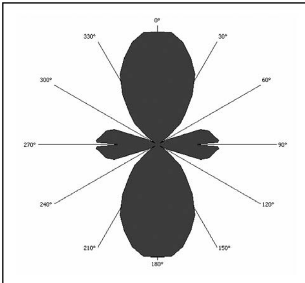
Fig 3: Wavefunction of the peak at about 8040Hz that belongs to the radial quantum number n' = 1 (left) and calculated spherical harmonics for l = 2, m = 0 (right).
