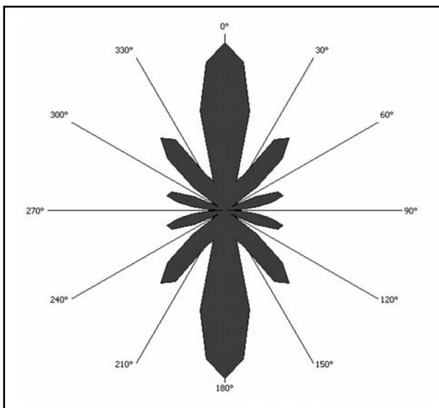
Fig 4: Wavefunction of the peak at about 7460Hz (left) and calculated spherical harmonics for l = 5, m = 0 (right).
