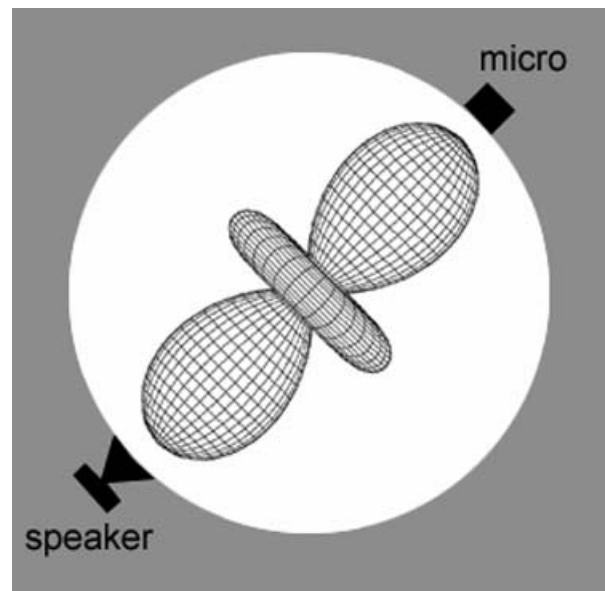
Fig 2: An inside "view" of the pressure wave.
